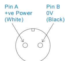
Connection Details
