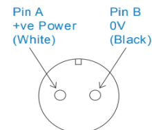
Connection Details
