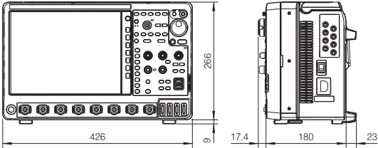
DLM5000/DLM5000HD
